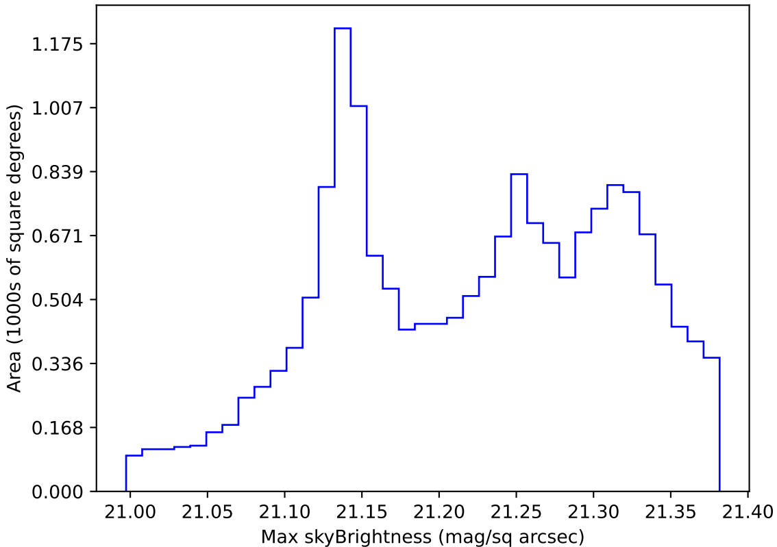
extra_ss_neo4_v3.4_10yrs WFD r band: Max skyBrightness
