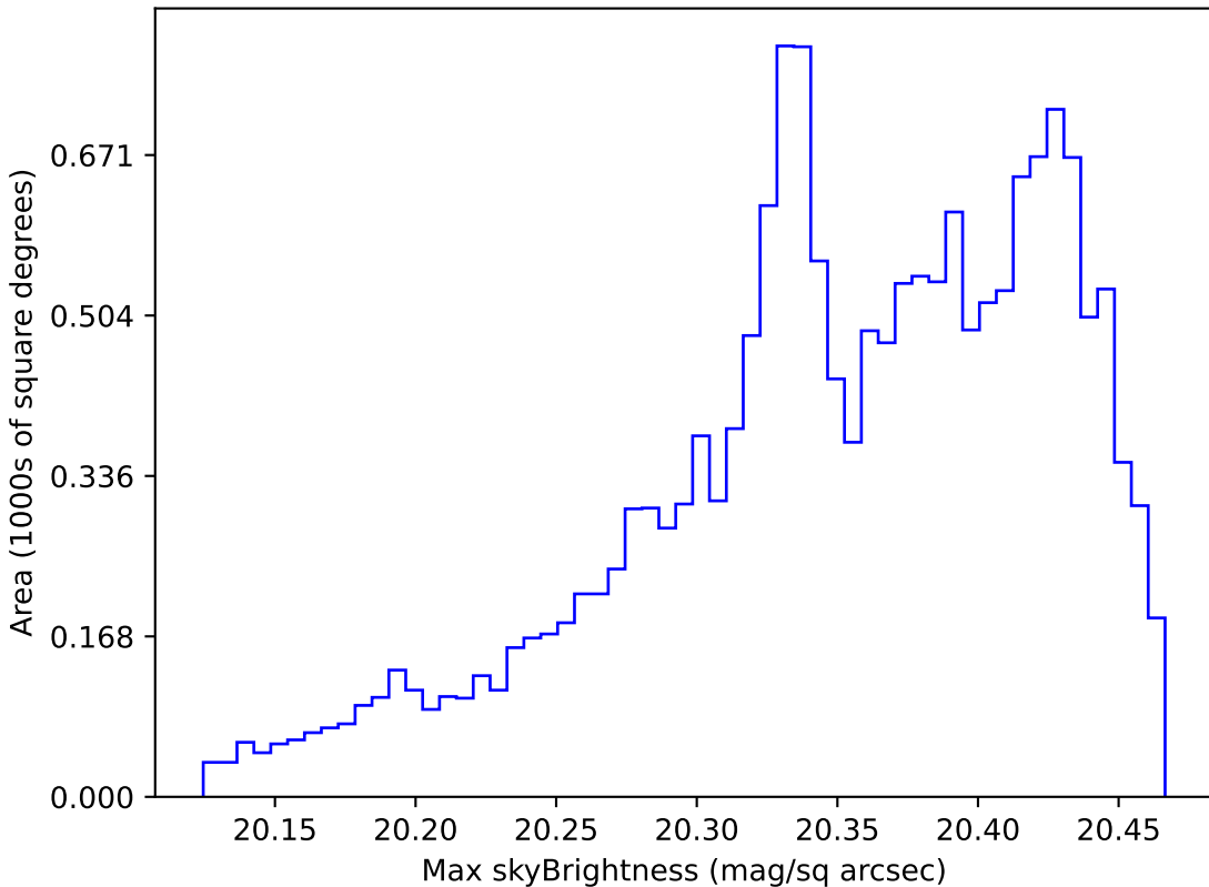
extra_ss_neo4_v3.4_10yrs WFD i band: Max skyBrightness
