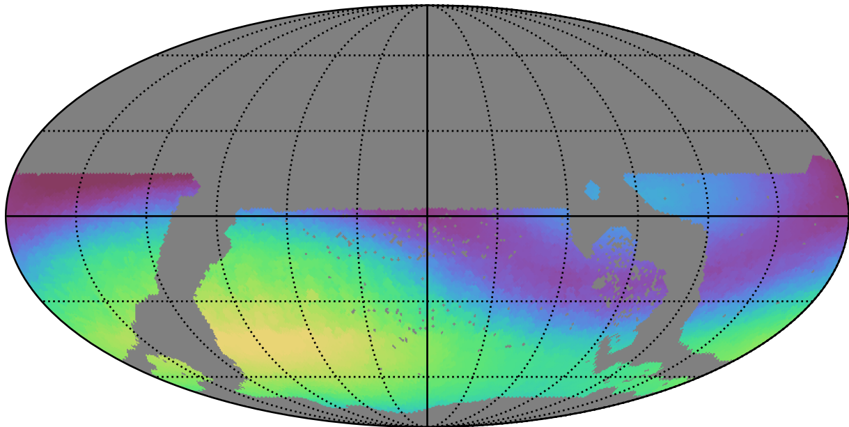
extra_ss_neo4_v3.4_10yrs WFD g band: Max skyBrightness
