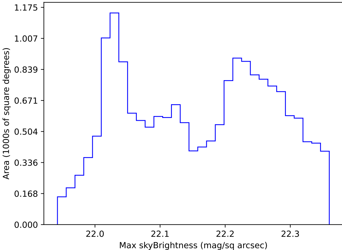
extra_ss_neo4_v3.4_10yrs WFD g band: Max skyBrightness
