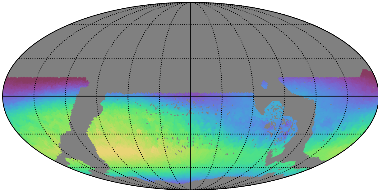
extra_ss_neo4_v3.4_10yrs WFD all bands: Max skyBrightness
