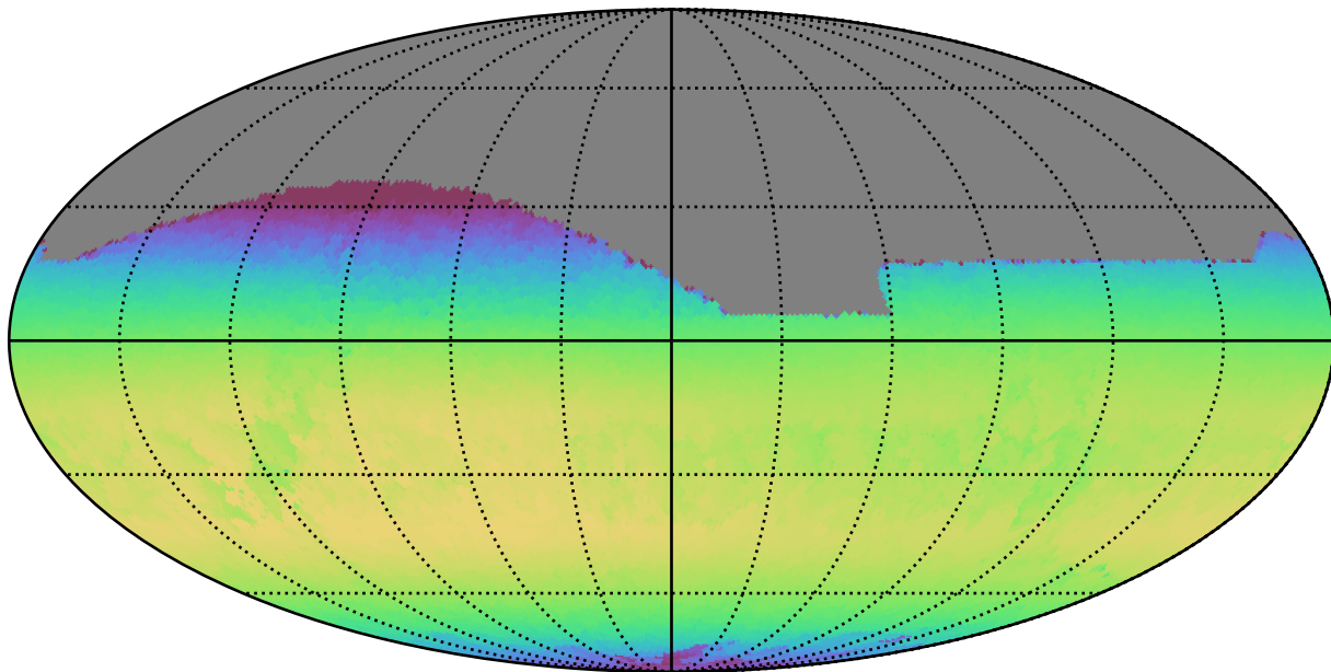
extra_ss_neo4_v3.4_10yrs All sky z band: Max skyBrightness
