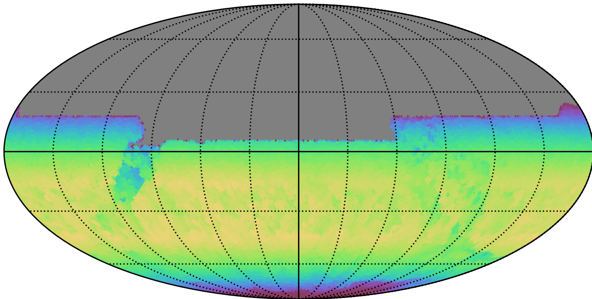
extra_ss_neo4_v3.4_10yrs All sky y band: Max skyBrightness
