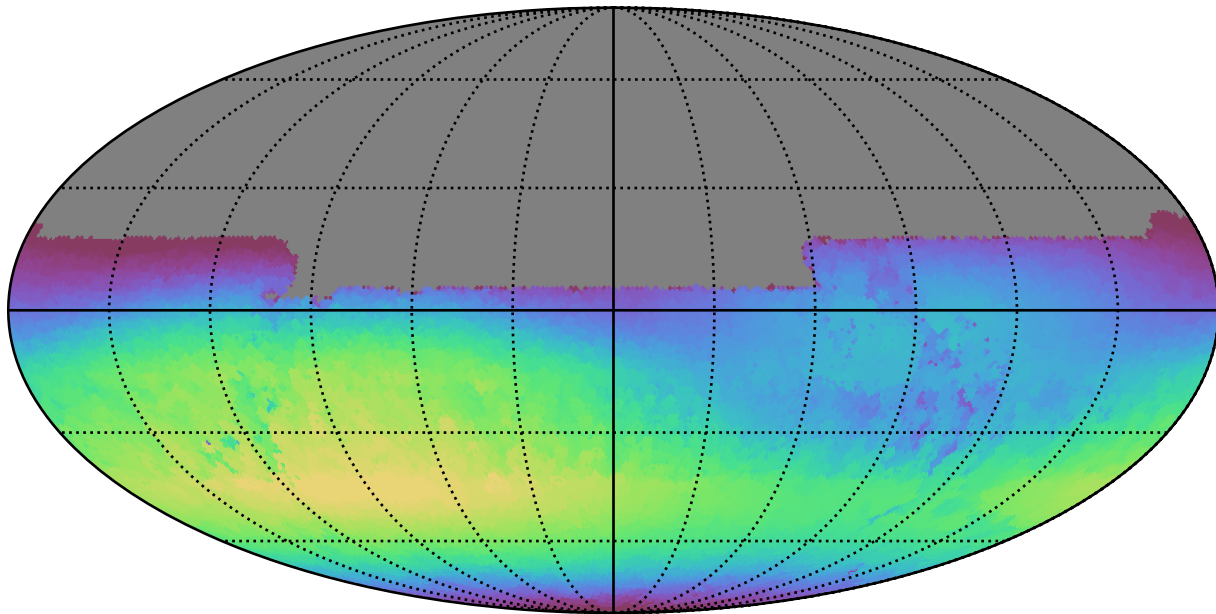
extra_ss_neo4_v3.4_10yrs All sky u band: Max skyBrightness
