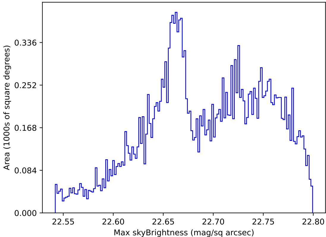
extra_ss_neo4_v3.4_10yrs All sky u band: Max skyBrightness
