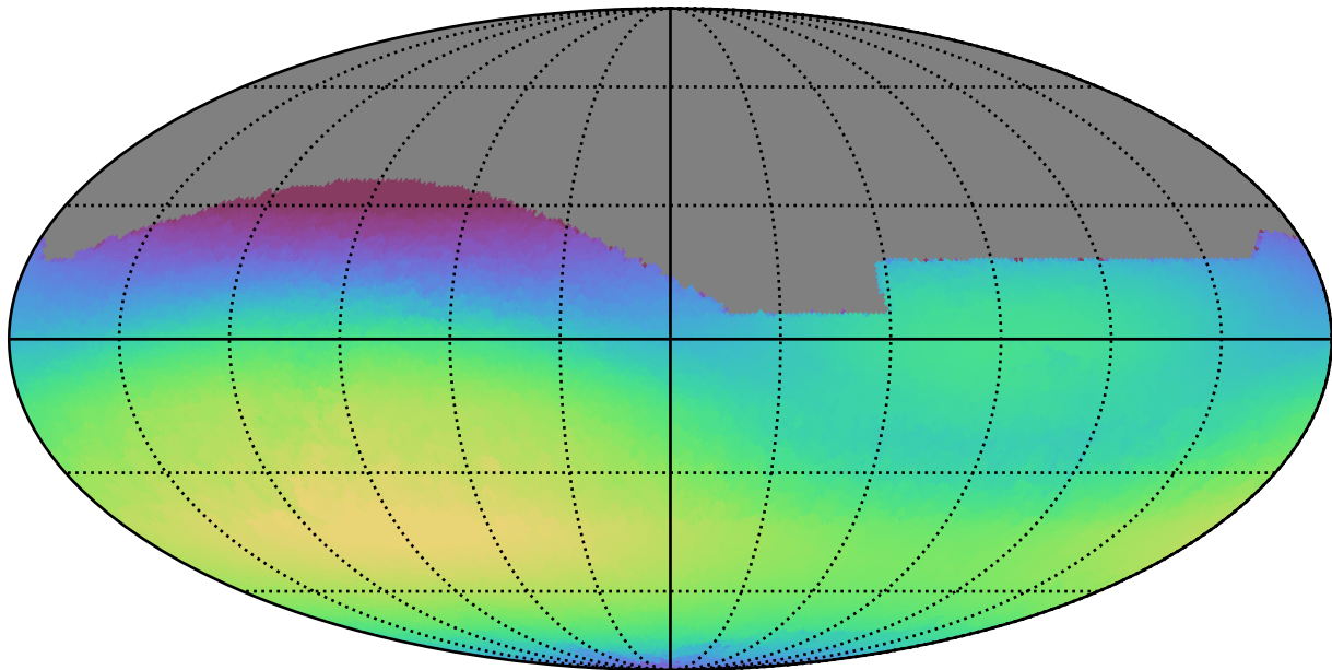
extra_ss_neo4_v3.4_10yrs All sky r band: Max skyBrightness
