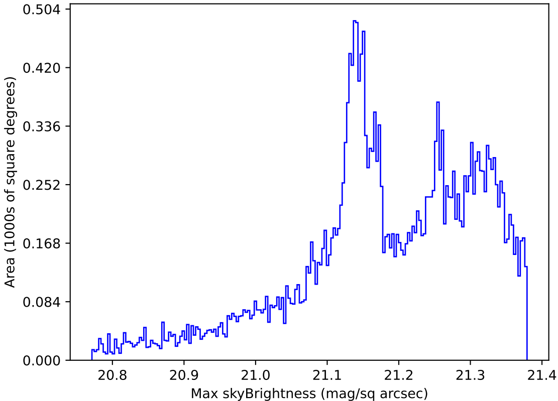
extra_ss_neo4_v3.4_10yrs All sky r band: Max skyBrightness
