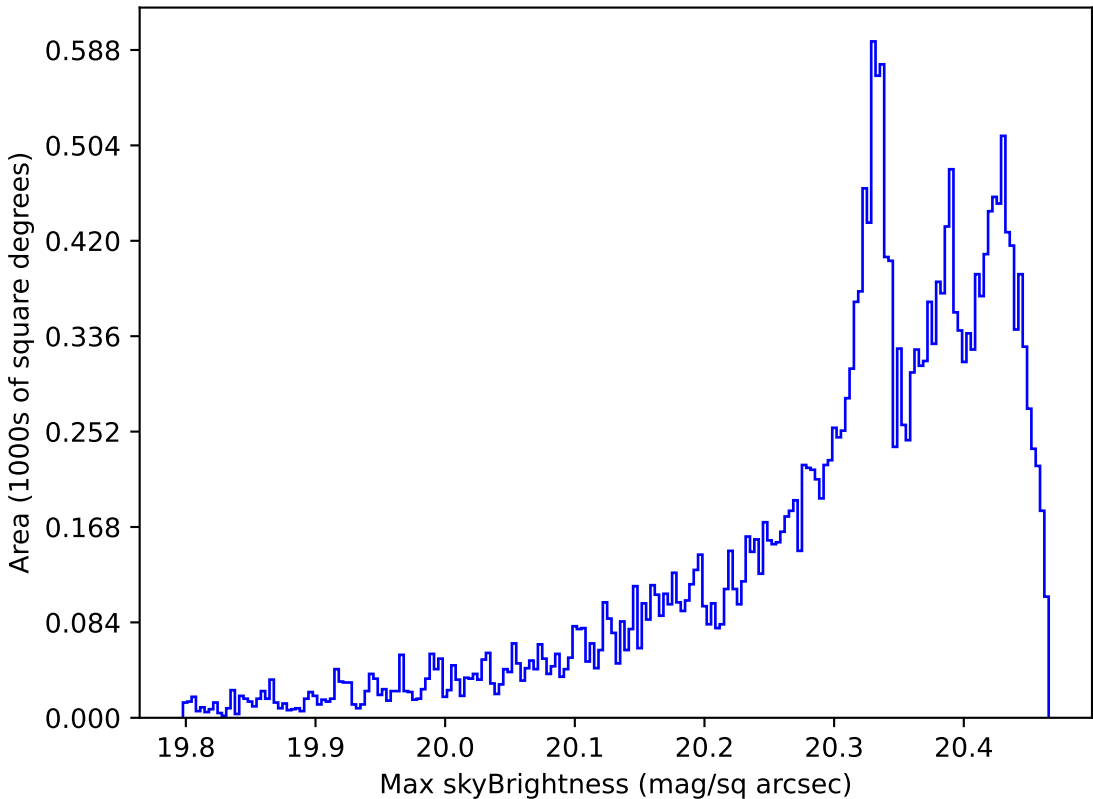
extra_ss_neo4_v3.4_10yrs All sky i band: Max skyBrightness
