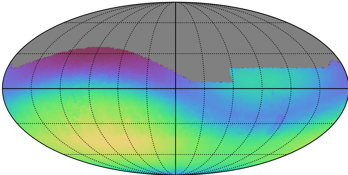
extra_ss_neo4_v3.4_10yrs All sky g band: Max skyBrightness
