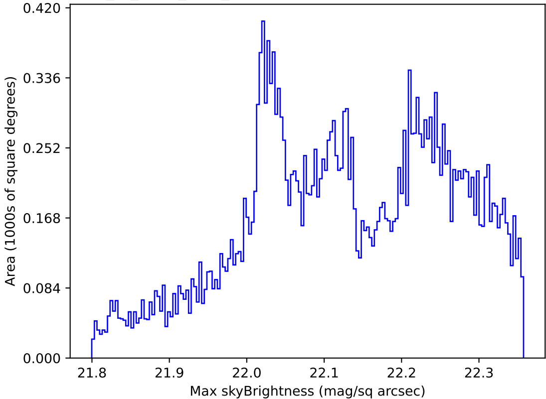
extra_ss_neo4_v3.4_10yrs All sky g band: Max skyBrightness
