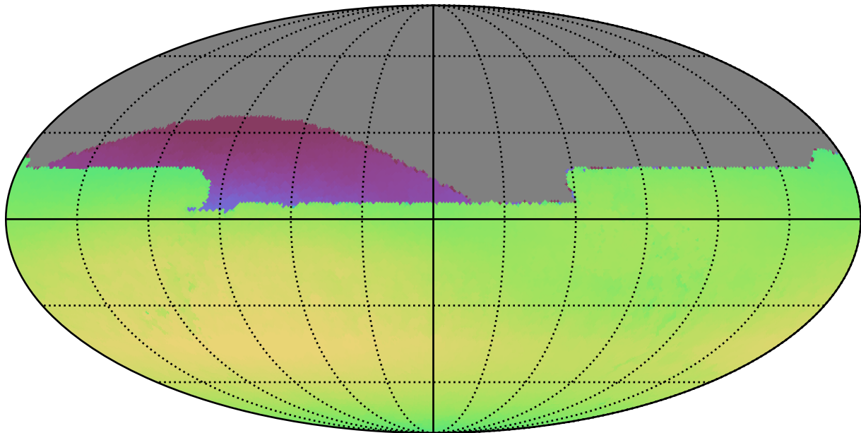
extra_ss_neo4_v3.4_10yrs All sky all bands: Max skyBrightness
