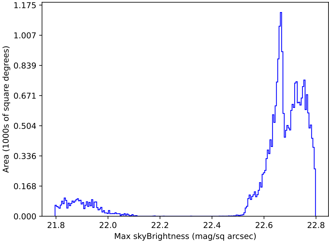
extra_ss_neo4_v3.4_10yrs All sky all bands: Max skyBrightness
