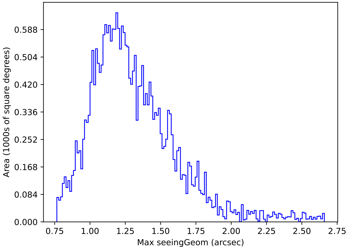
extra_ss_neo4_v3.4_10yrs Yr 1 z band: Max seeingGeom
