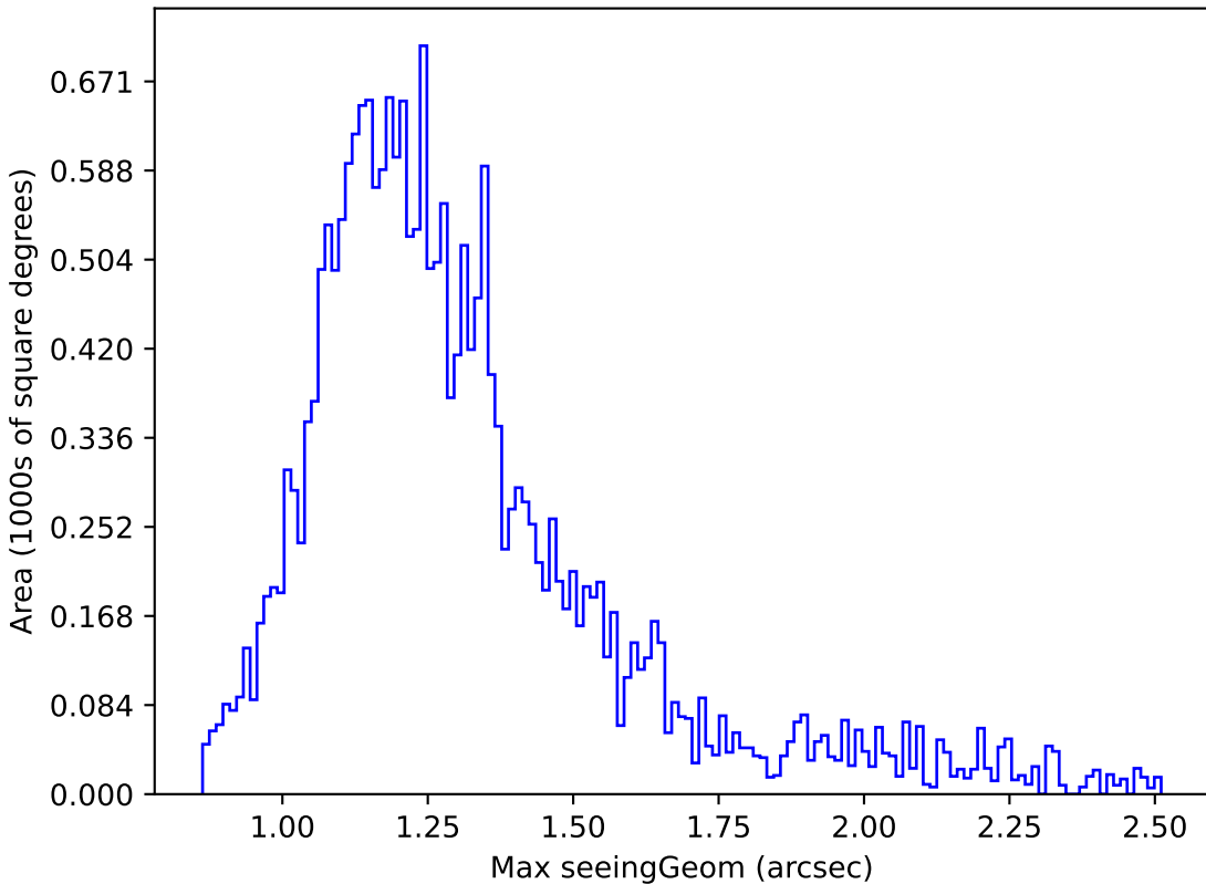
extra_ss_neo4_v3.4_10yrs Yr 1 y band: Max seeingGeom
