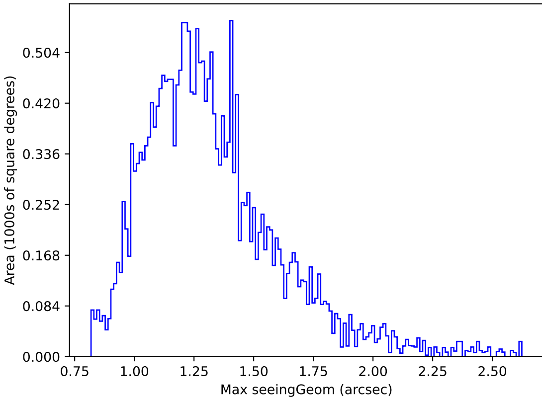
extra_ss_neo4_v3.4_10yrs Yr 1 u band: Max seeingGeom
