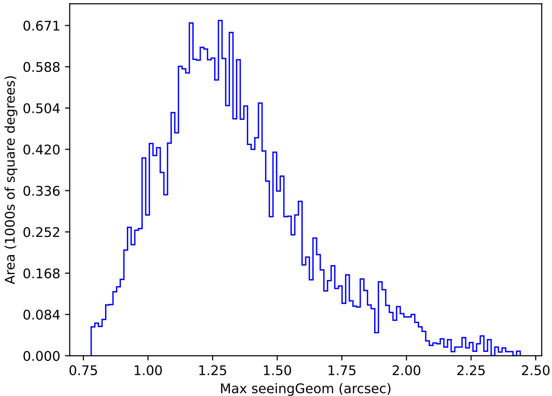
extra_ss_neo4_v3.4_10yrs Yr 1 r band: Max seeingGeom
