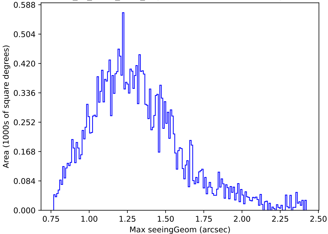
extra_ss_neo4_v3.4_10yrs Yr 1 i band: Max seeingGeom
