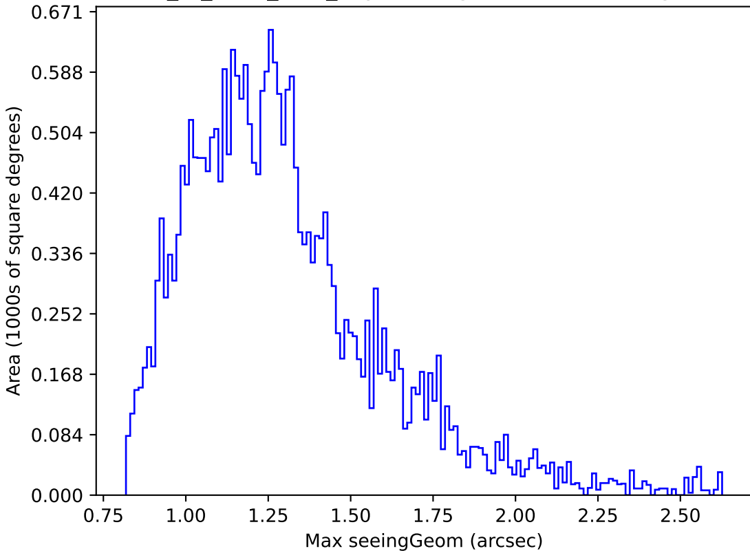
extra_ss_neo4_v3.4_10yrs Yr 1 g band: Max seeingGeom
