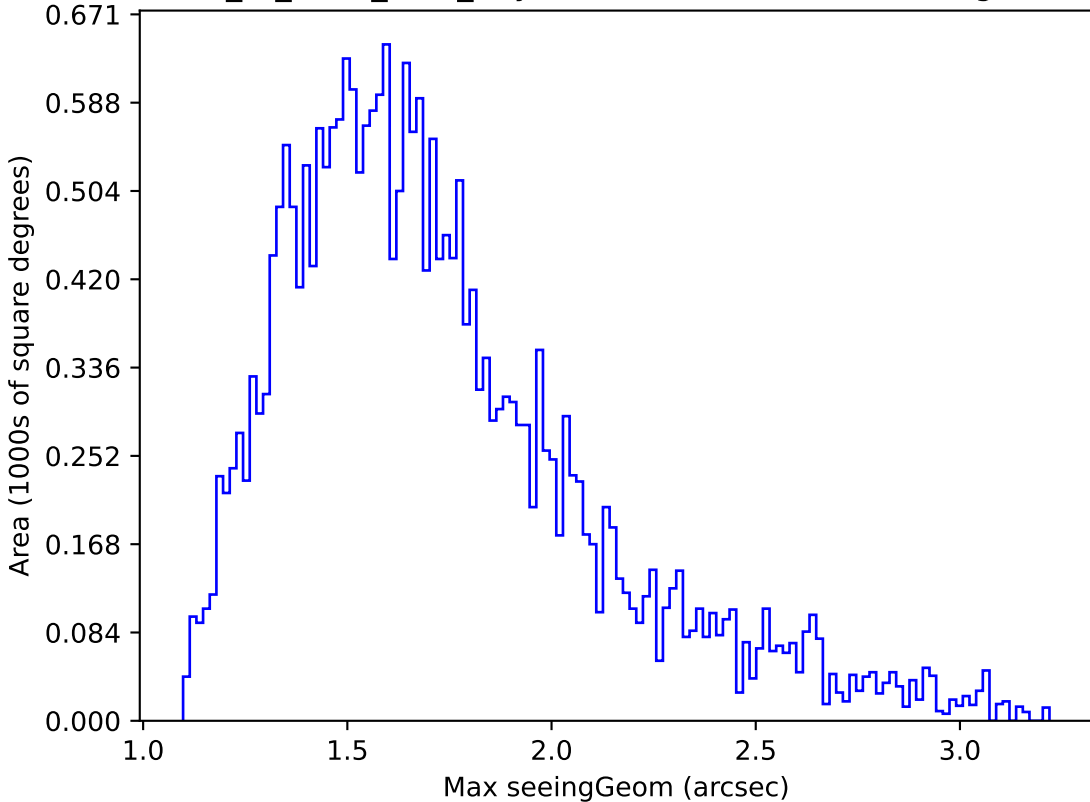
extra_ss_neo4_v3.4_10yrs Yr 1 all bands: Max seeingGeom
