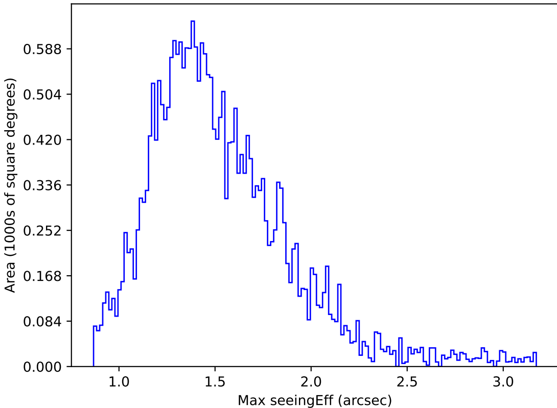
extra_ss_neo4_v3.4_10yrs Yr 1 z band: Max seeingEff
