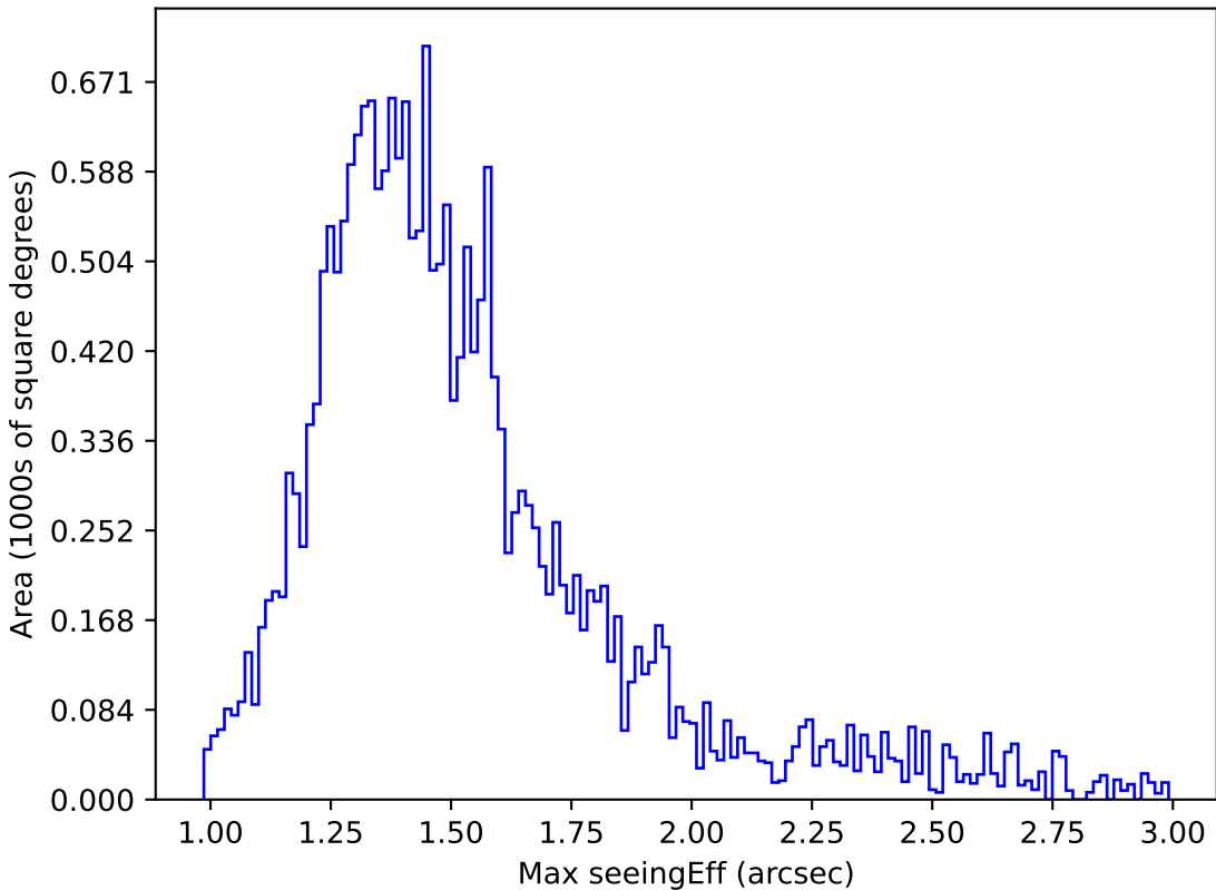
extra_ss_neo4_v3.4_10yrs Yr 1 y band: Max seeingEff
