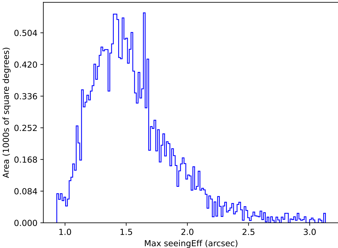
extra_ss_neo4_v3.4_10yrs Yr 1 u band: Max seeingEff
