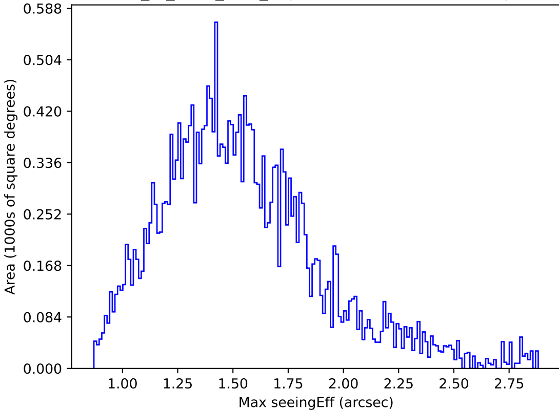
extra_ss_neo4_v3.4_10yrs Yr 1 i band: Max seeingEff
