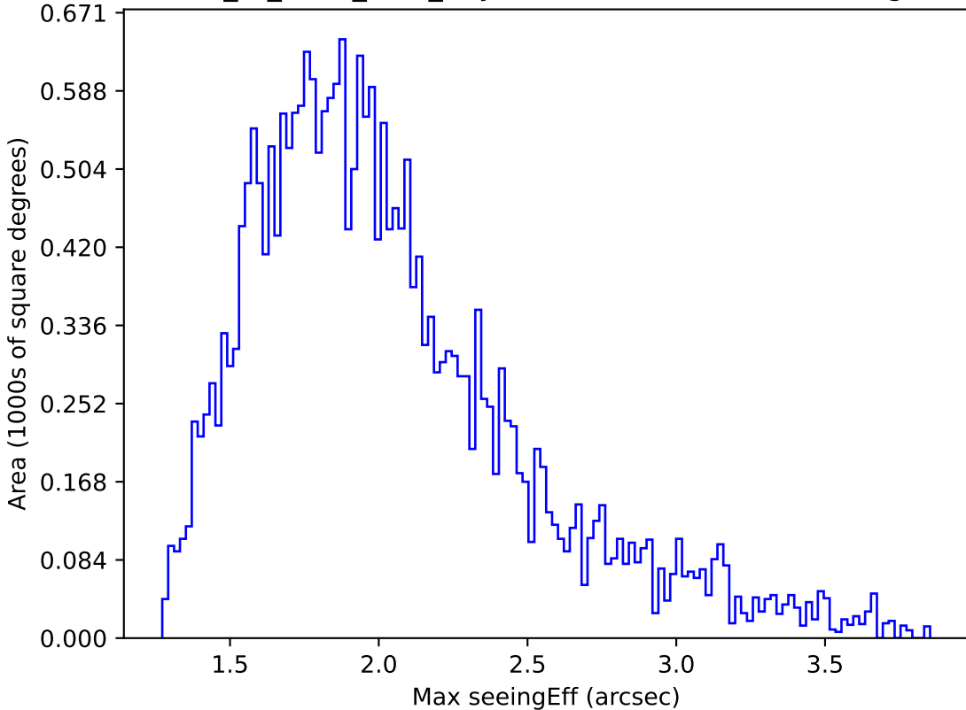
extra_ss_neo4_v3.4_10yrs Yr 1 all bands: Max seeingEff
