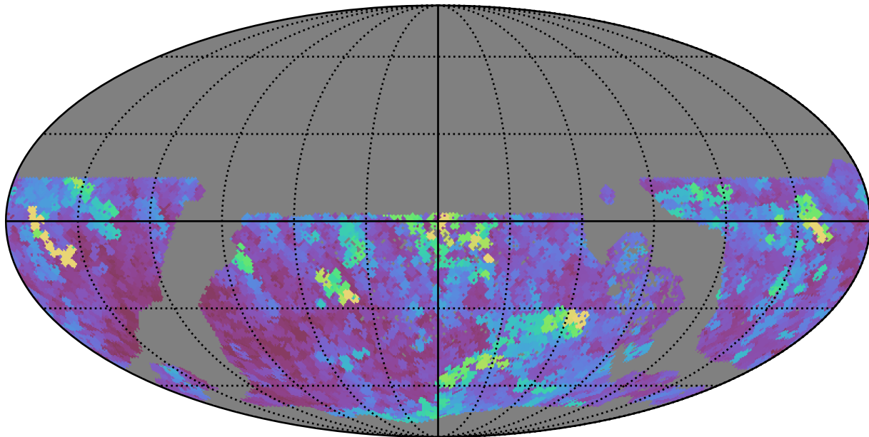
extra_ss_neo4_v3.4_10yrs WFD z band: Max seeingEff
