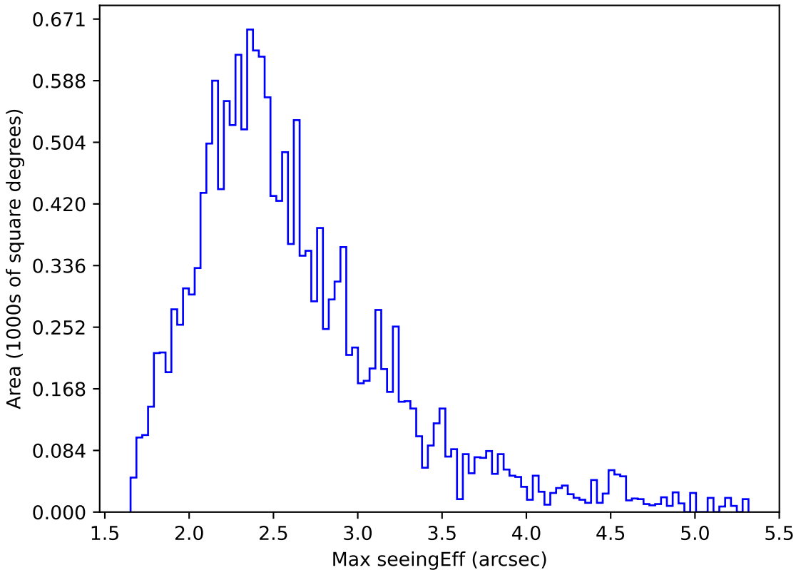
extra_ss_neo4_v3.4_10yrs WFD z band: Max seeingEff
