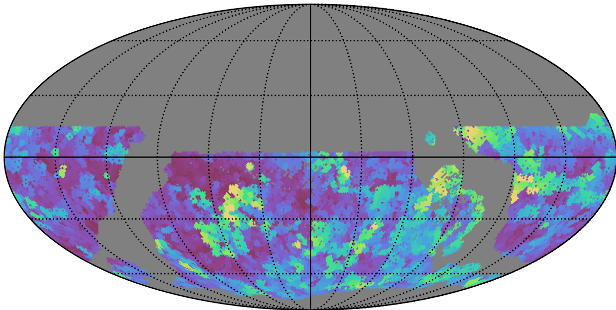
extra_ss_neo4_v3.4_10yrs WFD g band: Max seeingEff
