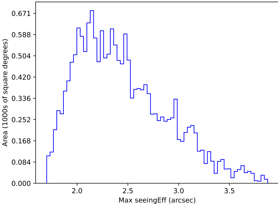
extra_ss_neo4_v3.4_10yrs WFD g band: Max seeingEff
