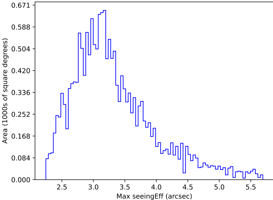
extra_ss_neo4_v3.4_10yrs WFD all bands: Max seeingEff
