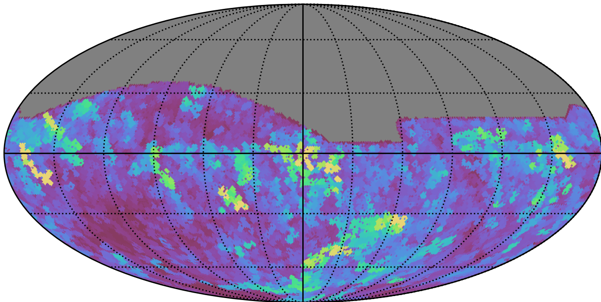
extra_ss_neo4_v3.4_10yrs All sky z band: Max seeingEff
