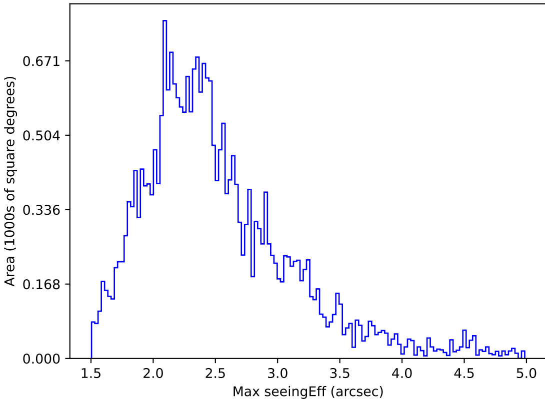
extra_ss_neo4_v3.4_10yrs All sky z band: Max seeingEff
