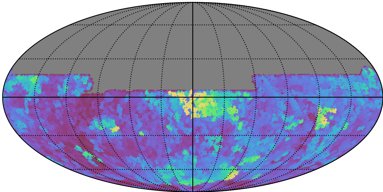
extra_ss_neo4_v3.4_10yrs All sky y band: Max seeingEff
