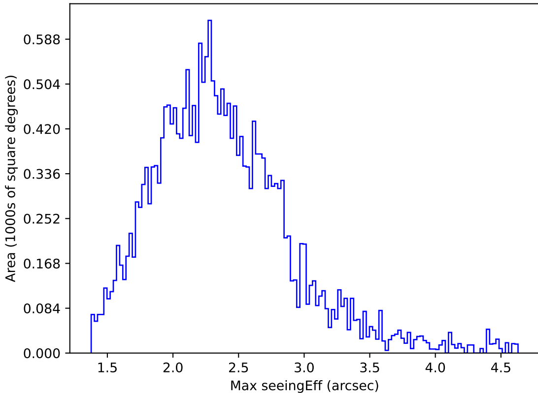
extra_ss_neo4_v3.4_10yrs All sky y band: Max seeingEff
