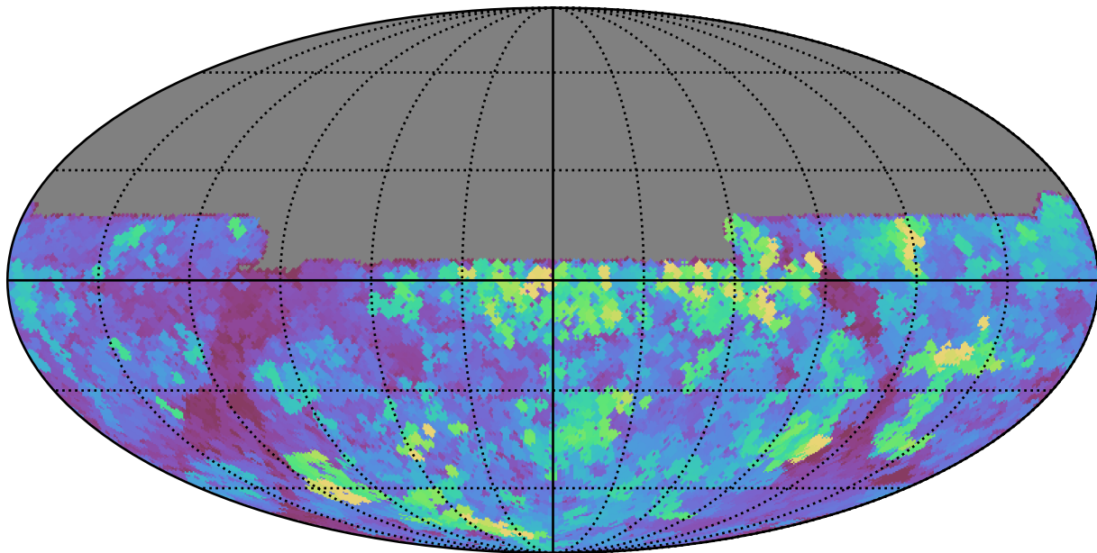
extra_ss_neo4_v3.4_10yrs All sky u band: Max seeingEff
