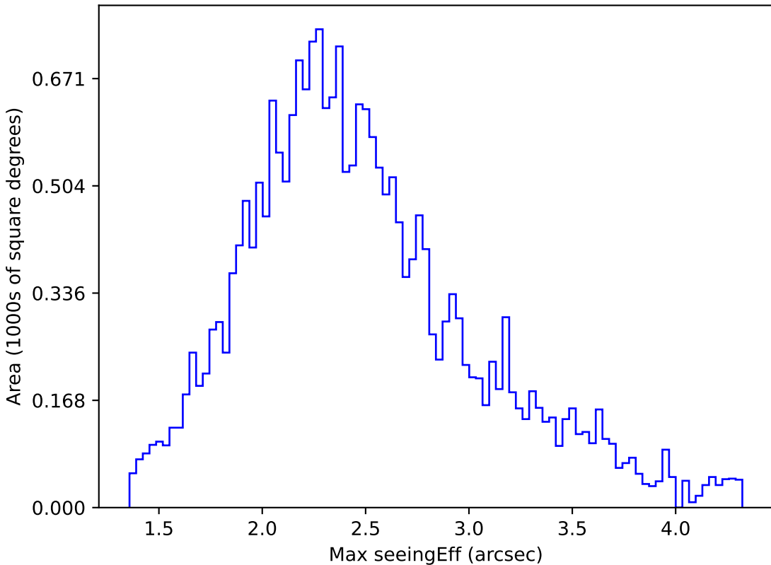
extra_ss_neo4_v3.4_10yrs All sky u band: Max seeingEff
