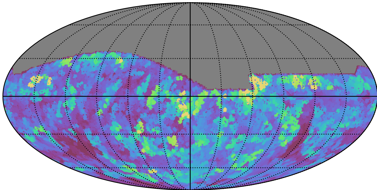
extra_ss_neo4_v3.4_10yrs All sky r band: Max seeingEff
