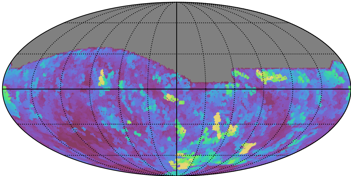
extra_ss_neo4_v3.4_10yrs All sky i band: Max seeingEff
