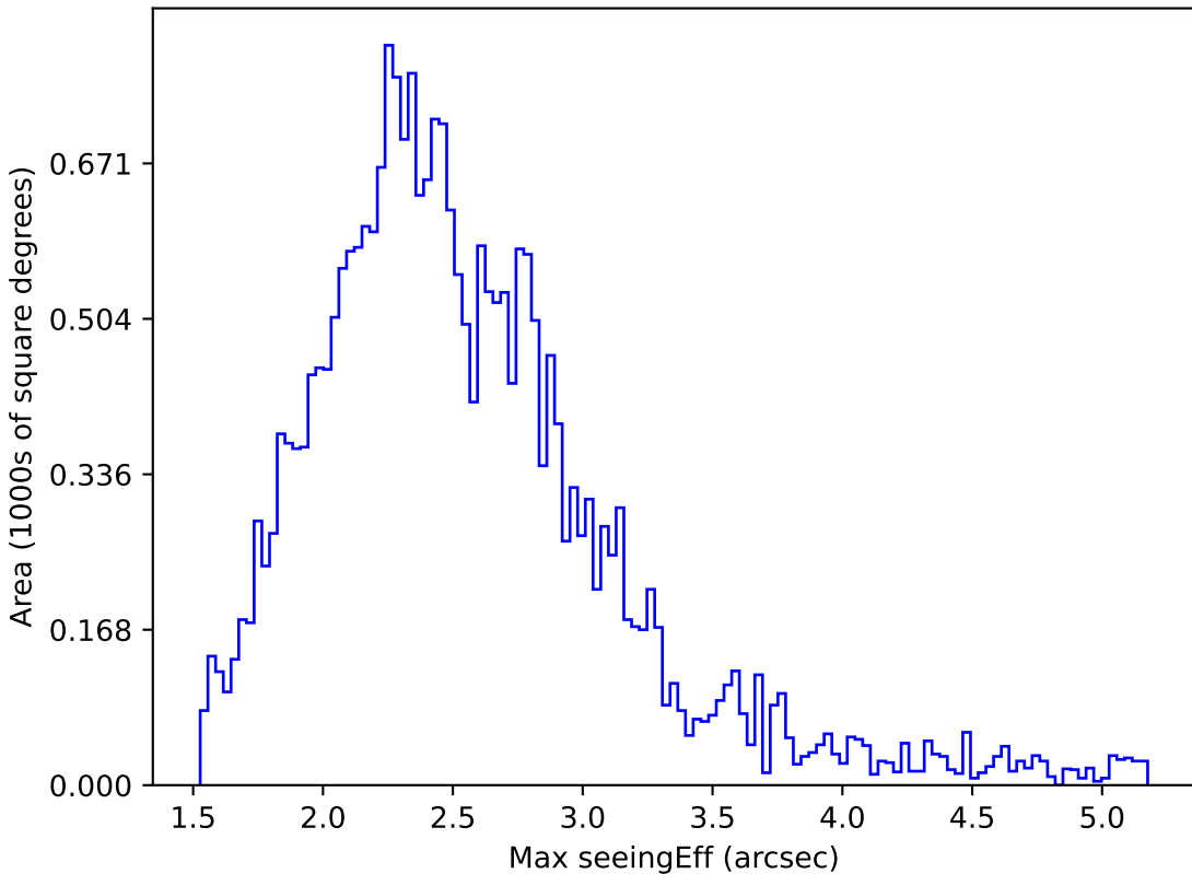
extra_ss_neo4_v3.4_10yrs All sky i band: Max seeingEff
