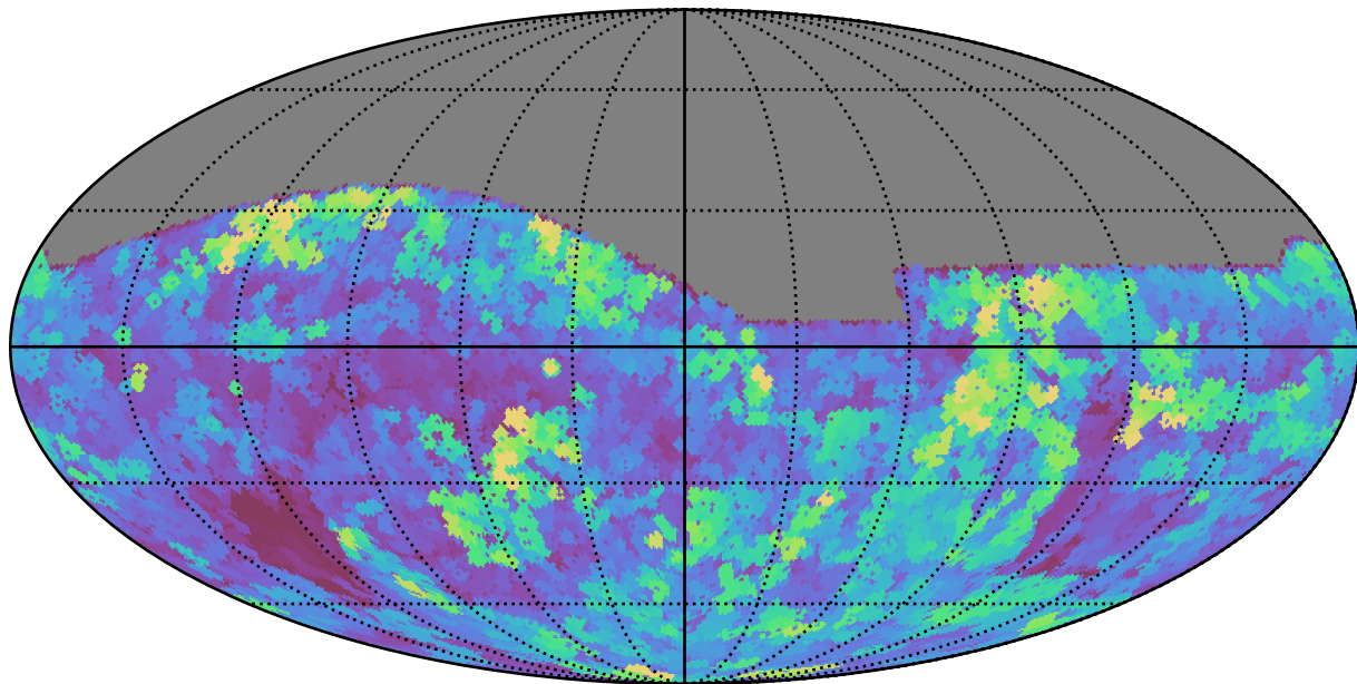
extra_ss_neo4_v3.4_10yrs All sky g band: Max seeingEff
