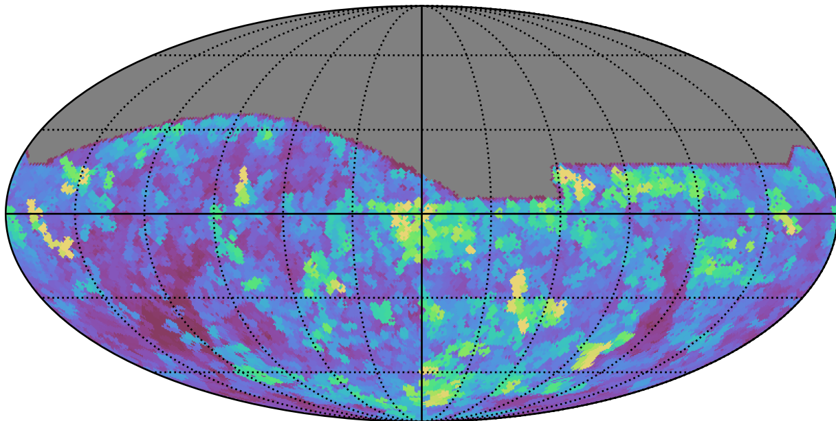
extra_ss_neo4_v3.4_10yrs All sky all bands: Max seeingEff
