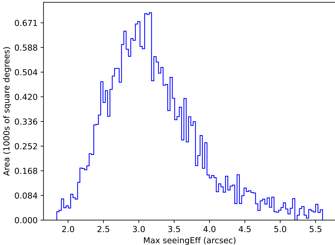
extra_ss_neo4_v3.4_10yrs All sky all bands: Max seeingEff
