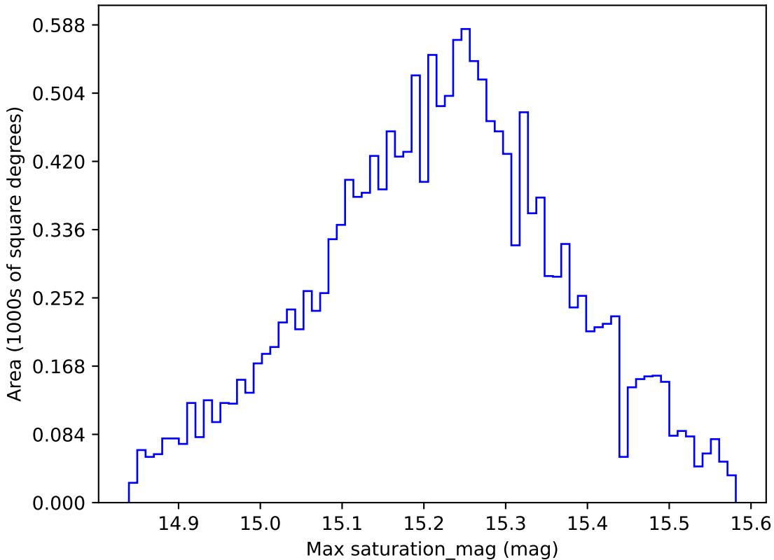
extra_ss_neo4_v3.4_10yrs WFD z band: Max saturation_mag
