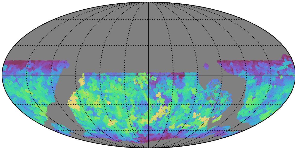
extra_ss_neo4_v3.4_10yrs WFD y band: Max saturation_mag
