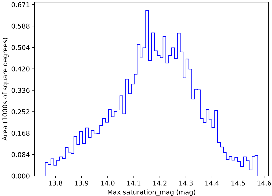
extra_ss_neo4_v3.4_10yrs WFD y band: Max saturation_mag
