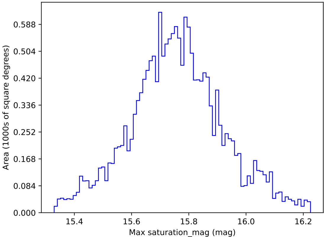
extra_ss_neo4_v3.4_10yrs WFD r band: Max saturation_mag
