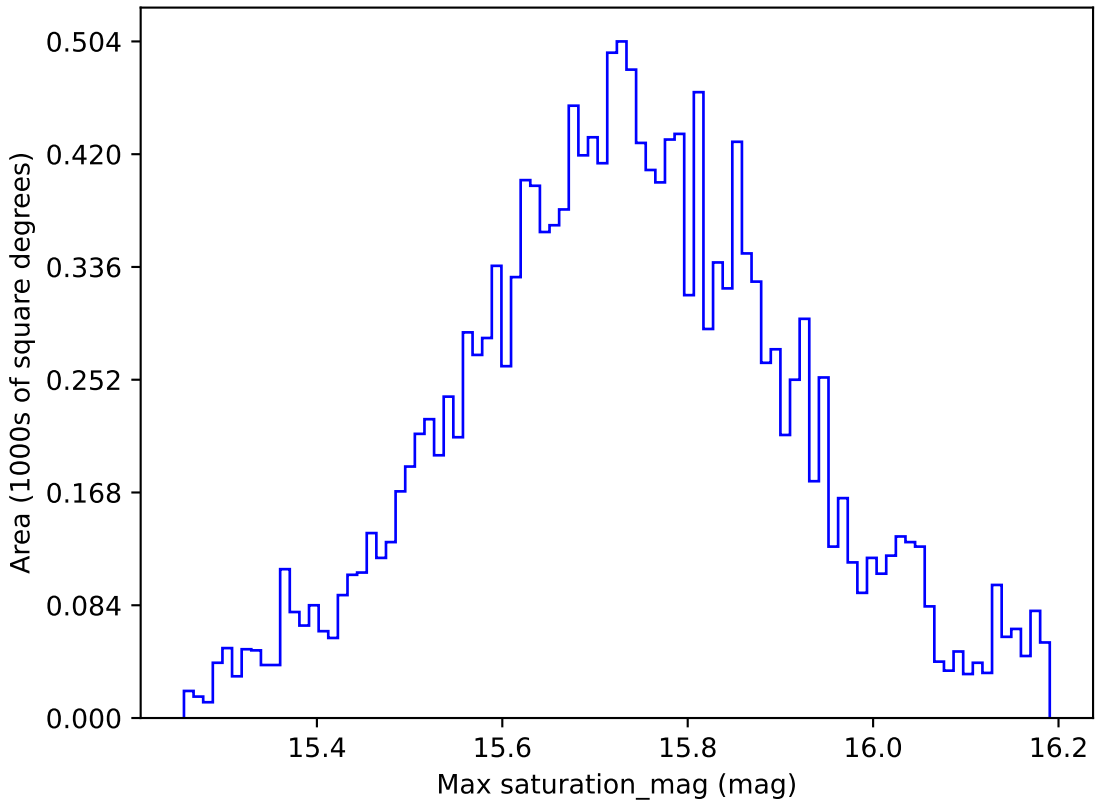
extra_ss_neo4_v3.4_10yrs WFD g band: Max saturation_mag
